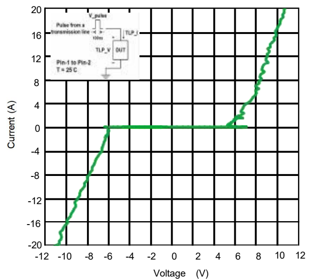
Fig 6. TLP Measurement
