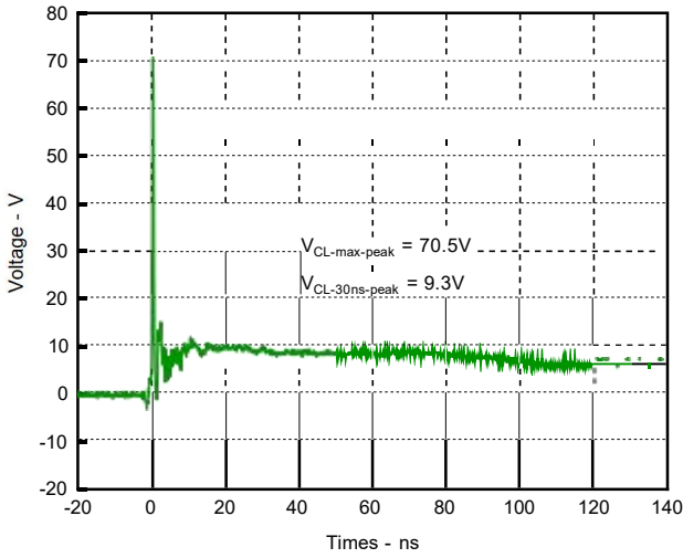
Fig 7. Clamping Voltage at IEC61000-4-2 +8kV Pulse Waveform
