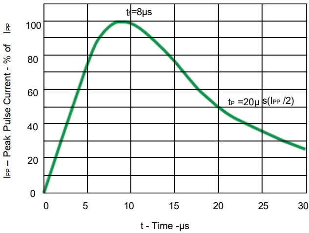
Fig 1. Pulse Waveform
